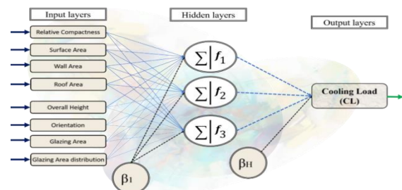
Figure 7: The general structure of the MLP
