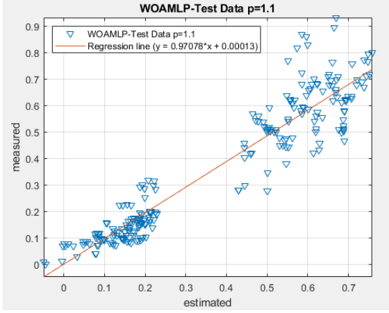
(g) WOAMLP test \alpha=1.1
