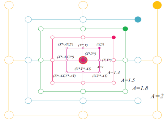
Figure 11: WOA algorithm's Exploration mechanism.
